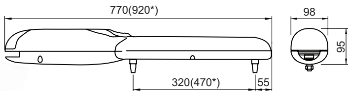
*WG3524, WG3524HS
